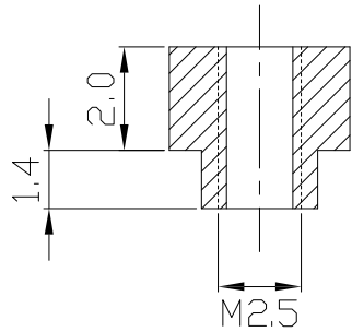
sectional drawing A-A
