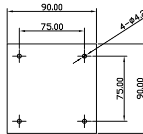
PCB LAYOUT
