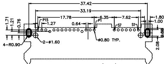
P.C.B LAYOUT (T=1.2) TOP VIEW
