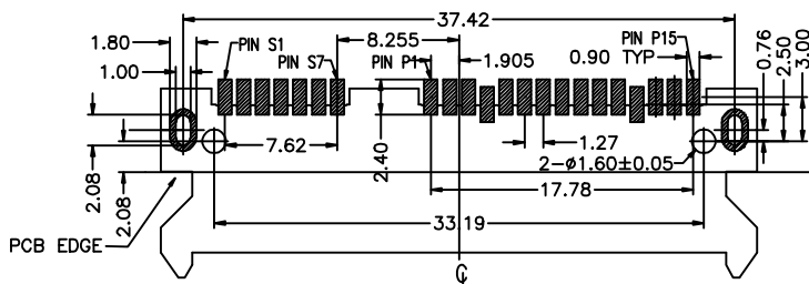
P.C.B LAYOUT (T=1.20) TOP VIEW
