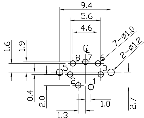
COMPONENT SIDE (PCB LAYOUT)
