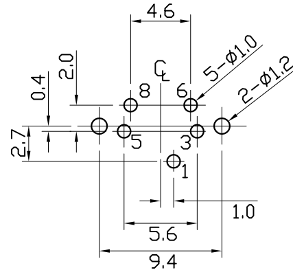
COMPONENT SIDE (PCB LAYOUT)
