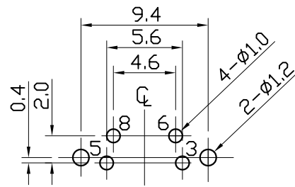
COMPONENT SIDE (PCB LAYOUT)
