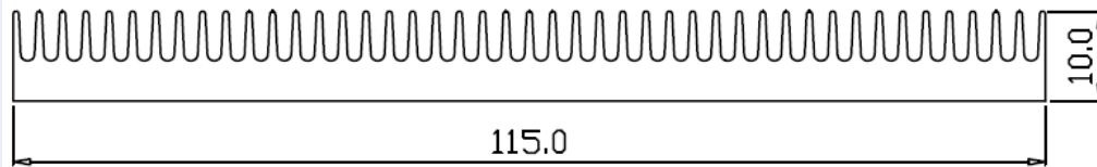
Series Number: RG-9A170 Dimension(mm): 115x10.0xFree
