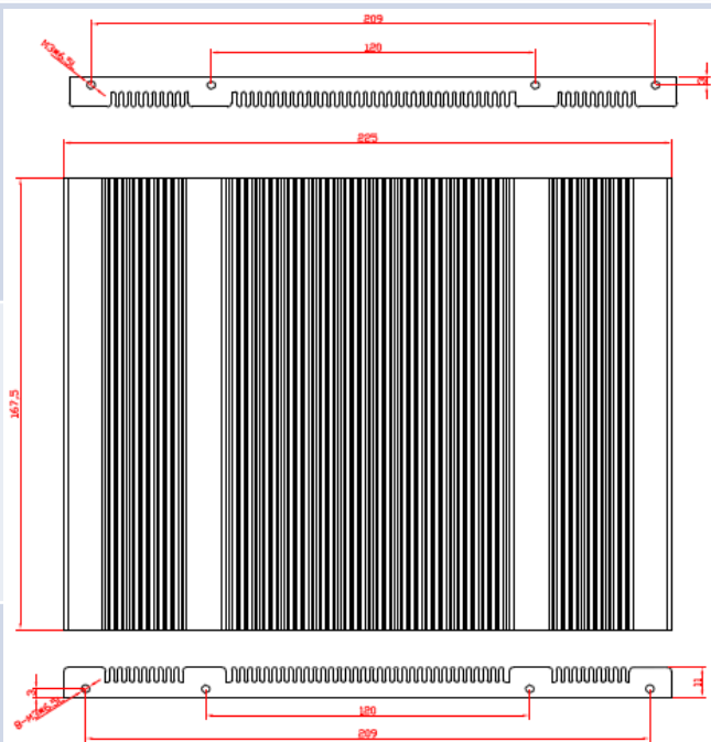
Series Number: RG-NC336 Dimension(mm): 225.0x11.0x167.5
