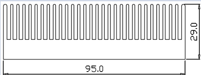
Series Number: RG-8E253 Dimension(mm): 95.0x29.0xFree
