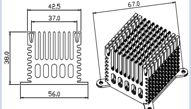
Series Number: RG-CM430X Dimension(mm): 56.0x38.0xFree
