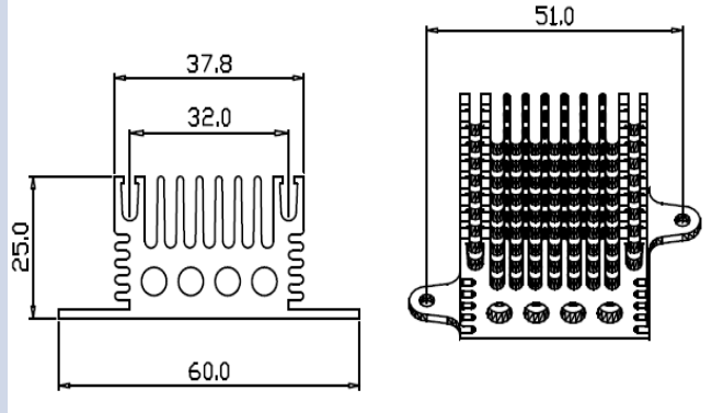
Series Number: RG-CM378 Dimension(mm): 60.0x25.0xFree
