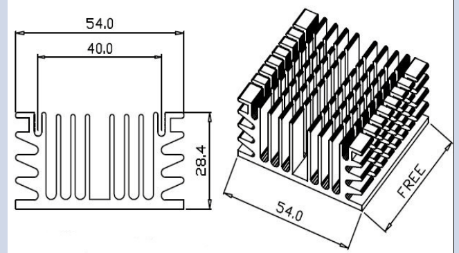
Series Number: RG-CM448 Dimension(mm): 54.0x28.4xFree
