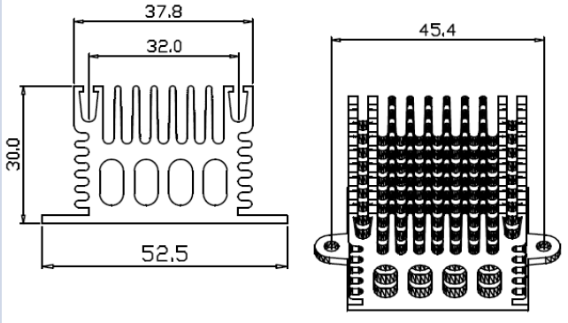
Series Number: RG-CM435 Dimension(mm): 52.5x30.0xFree
