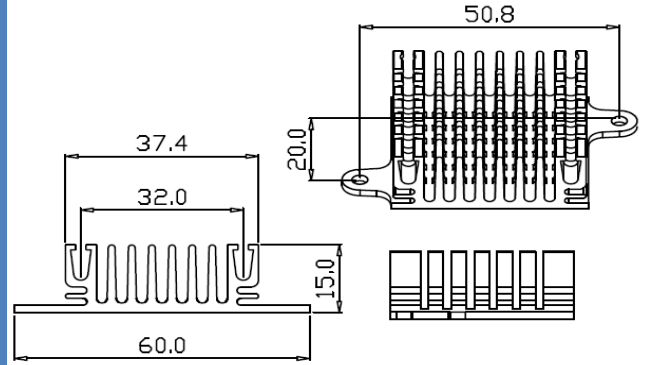
Series Number: RG-CM489 Dimension(mm): 60.0x15.0xFree
