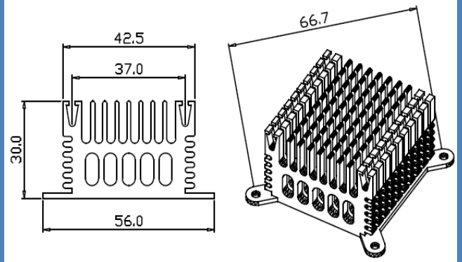
Series Number: RG-CM417X Dimension(mm): 56.0x30.0xFree
