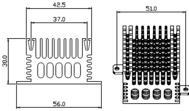
Series Number: RG-CM417A Dimension(mm): 56.0x30.0xFree
