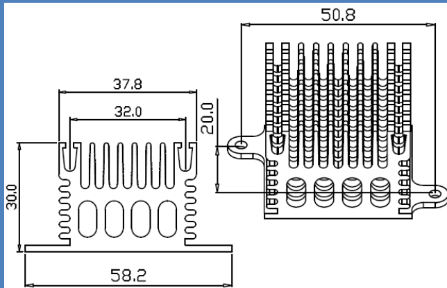
Series Number: RG-CM435A Dimension(mm): 58.2x30.0xFree
