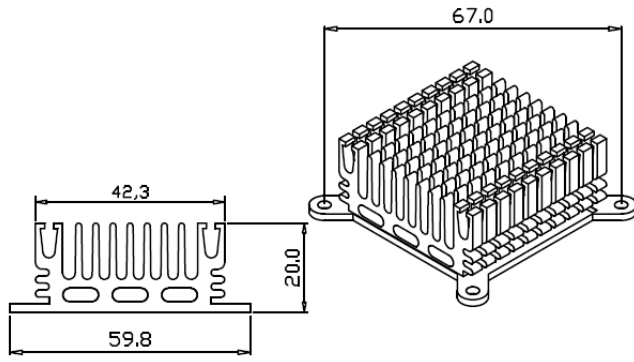
Series Number: RG-CM467X Dimension(mm): 59.8x20.0xFree
