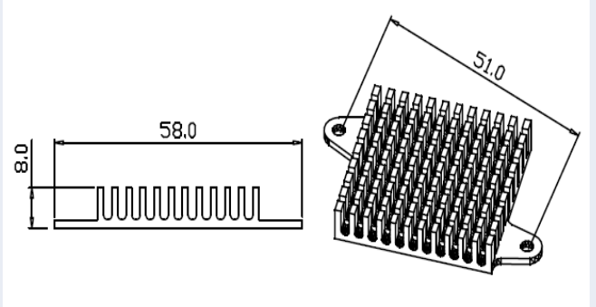
Series Number: RG-CM344 Dimension(mm): 58.0x8.0xFree
