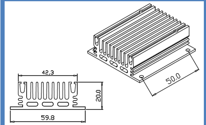
Series Number: RG-CM467-60W Dimension(mm): 59.8x20.0xFree
