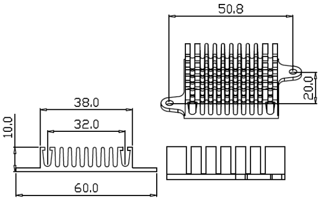
Series Number: RG-CM477B Dimension(mm): 60.0x10.0xFree
