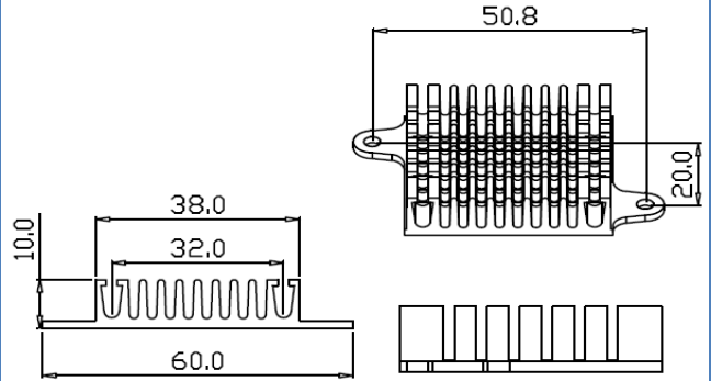
Series Number: RG-CM477A Dimension(mm): 60.0x10.0xFree
