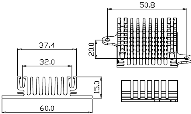
Series Number: RG-CM489A Dimension(mm): 60.0x15.0xFree
