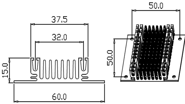
Series Number: RG-CM373-60W Dimension(mm): 60.0x15.0xFree
