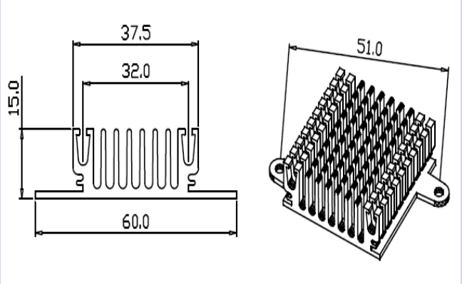
Series Number: RG-CM373 Dimension(mm): 60.0x15.0xFree
