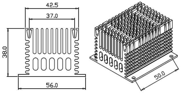
Series Number: RG-CM430-60W Dimension(mm): 56.0x38.0xFree
