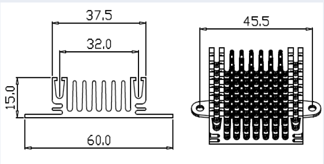
Series Number: RG-CM373 Dimension(mm): 60.0x15.0xFree
