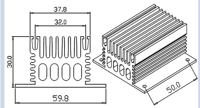
Series Number: RG-CM435-60W Dimension(mm): 59.8x30.0xFree
