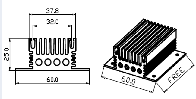
Series Number: RG-CM378 Dimension(mm): 60.0x25.0xFree
