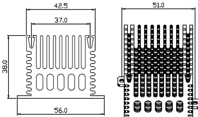
Series Number: RG-CM430A Dimension(mm): 56.0x38.0xFree
