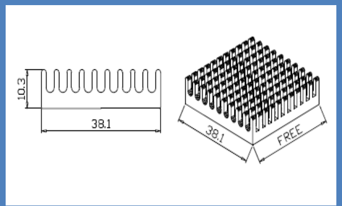
Series Number: RG-CM393 Dimension(mm): 38.1x10.3xFree
