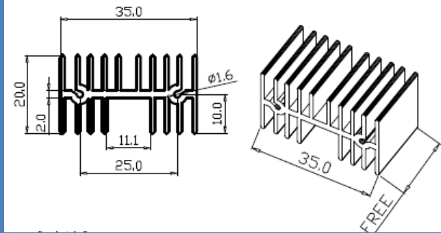
Series Number: RG-CM236 Dimension(mm): 35.0x20.0xFree
