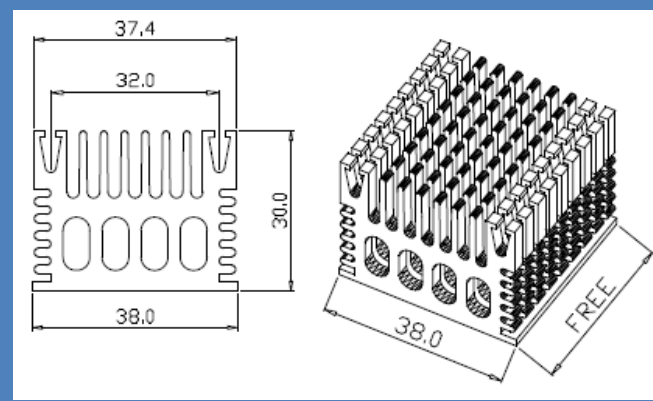
Series Number: RG-CM391E Dimension(mm): 38.0x30.0xFree
