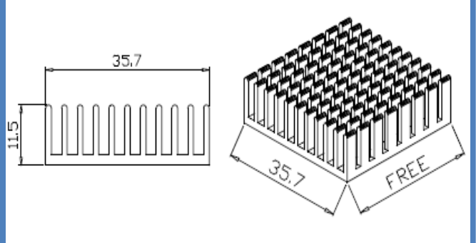
Series Number: RG-CM427 Dimension(mm): 35.7x11.5xFree
