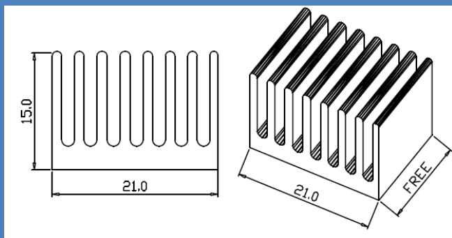
Series Number: RG-CM423 Dimension(mm): 21.0x15.0xFree
