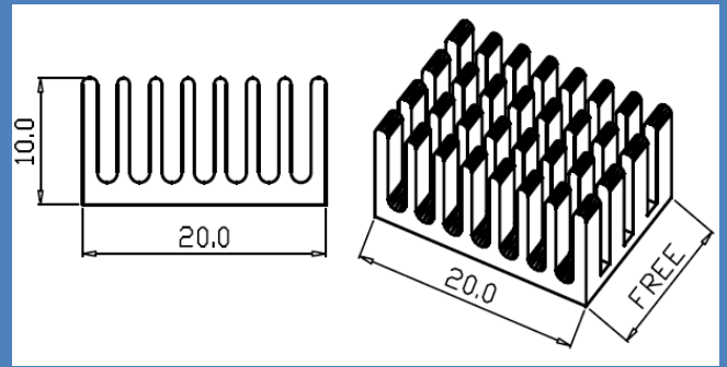
Series Number: RG-CM365CUT Dimension(mm): 20.0x10.0xFree
