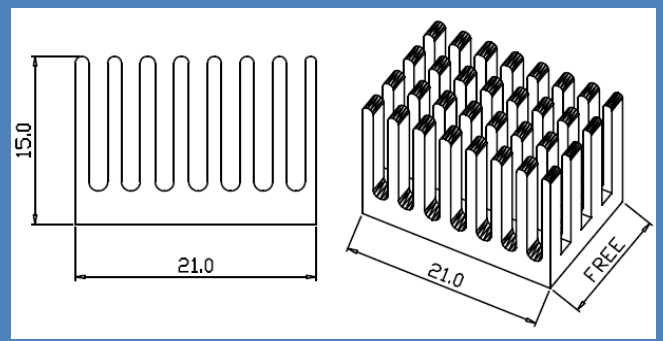
Series Number: RG-CM423CUT Dimension(mm): 21.0x15.0xFree
